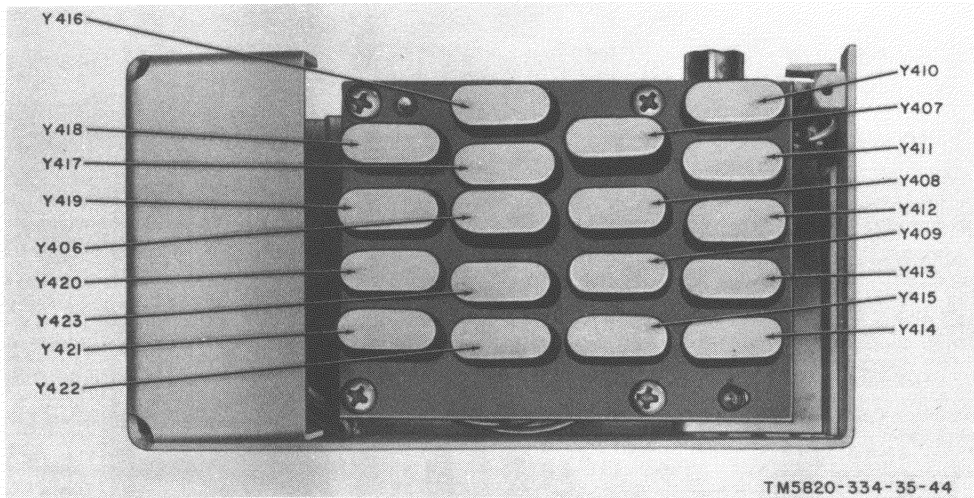
Figure 48. Crystal oscillator subchassis, left side view, cover removed.
