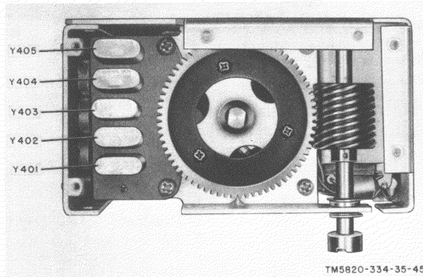
Figure 49. Crystal oscillator subchassis, right side view, cover removed.
