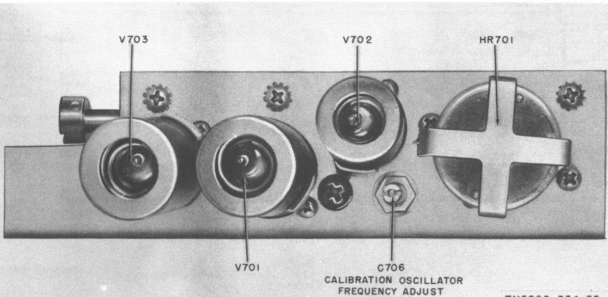
Figure 50. Calibration oscillator subchassis, top view.
