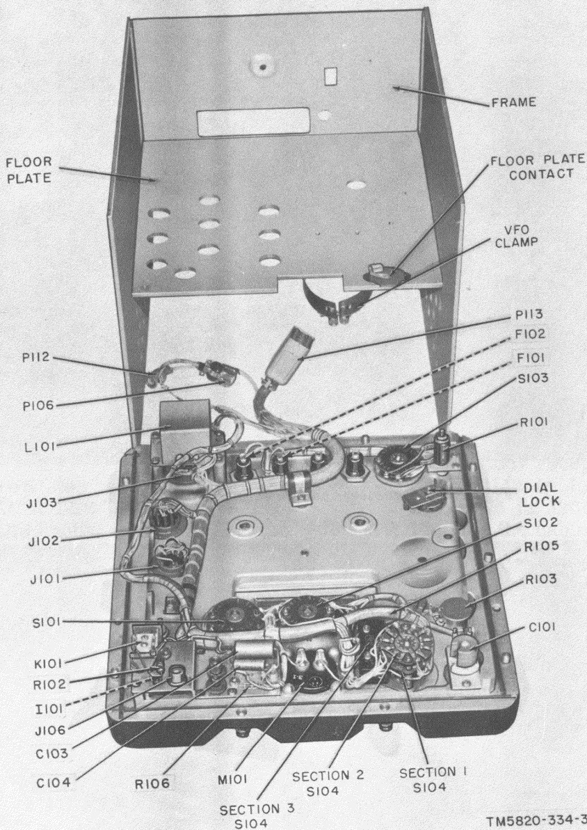
Figure 55. Front panel assembly, rear view.
