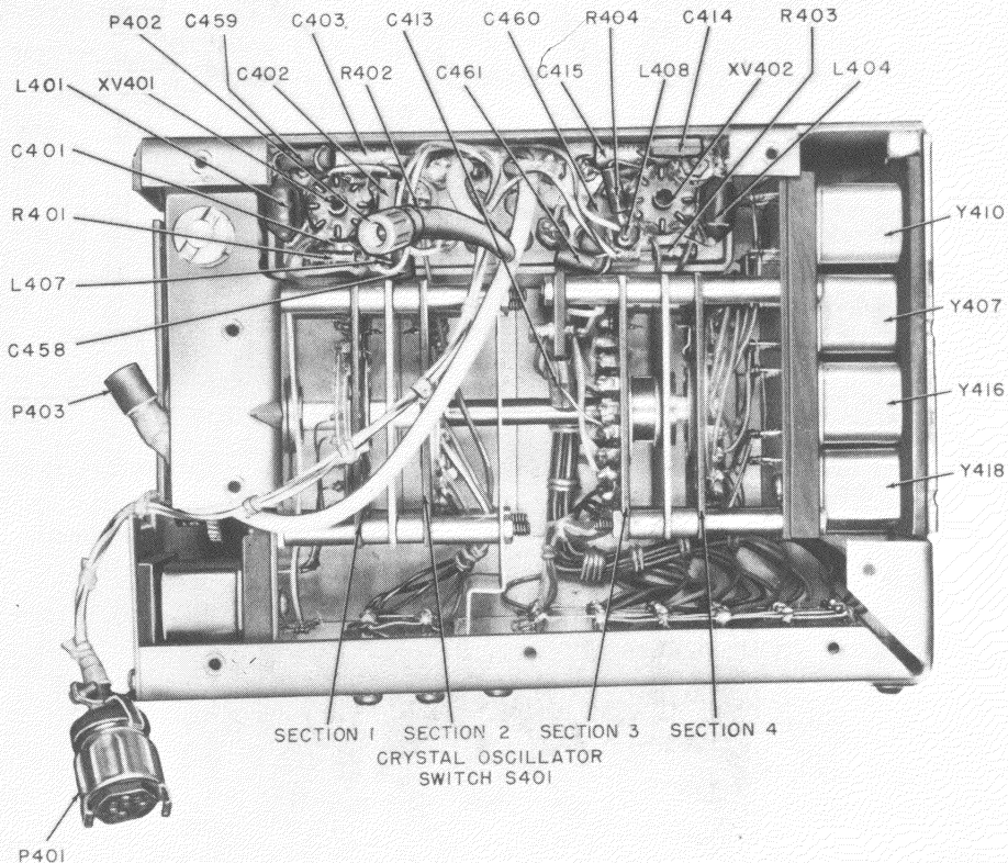
Figure 46. Crystal oscillator subchassis, front view, cover removed.
